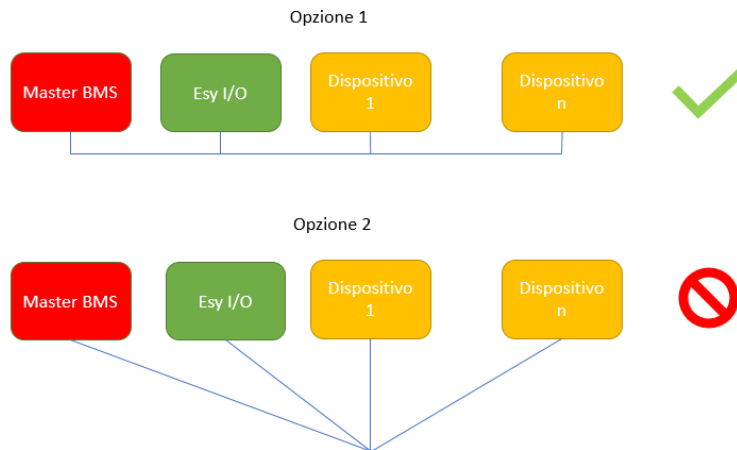
Figure 11: Examples of bus wiring
