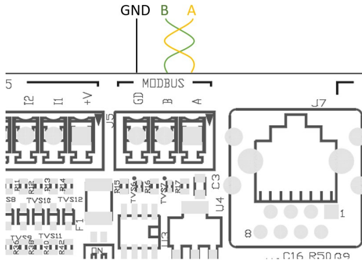
Figure 7: Câblage Rs485 Modbus
